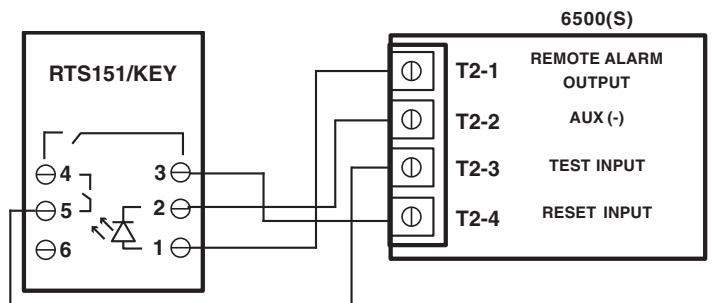
Figure 4: RTS151KEY Wiring
