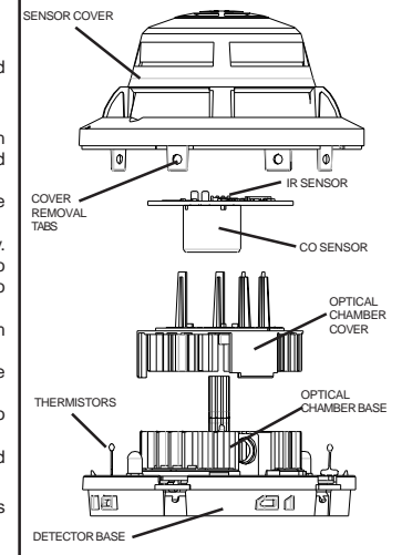
Figure 3: Sensor with Cover Removed
