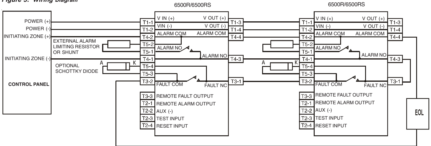
Figure 5: Wiring Diagram
