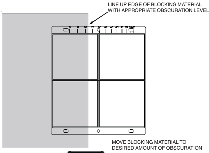
Figure 10. Reflector Test Card Procedure
