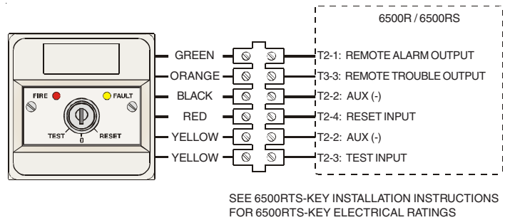
Figure 4: 6500RTS-KEY Wiring
