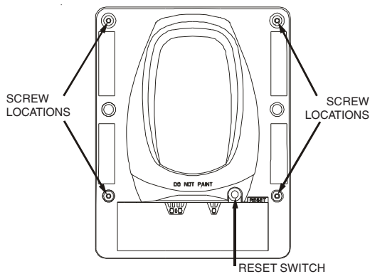
Figure 9: Housing Screw Locations
