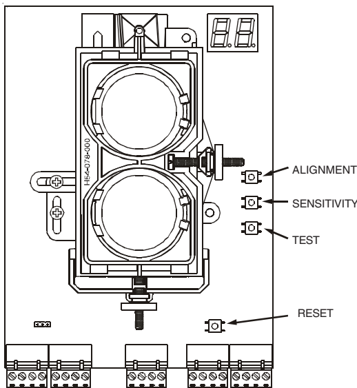
Figure 6: Switch Locations
