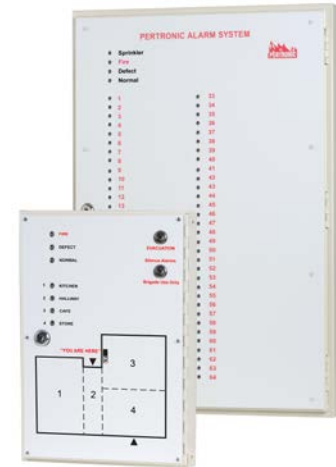
Slim Large FS Mimic Cabinet + Index with 64 zones without BCO & Evac (SLCABL PFS)
