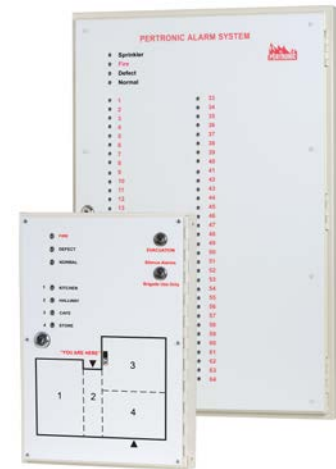
Slim Large FS Mimic Cabinet + Index with 64 zones without BCO & Evac (SLCABLPPFS)
