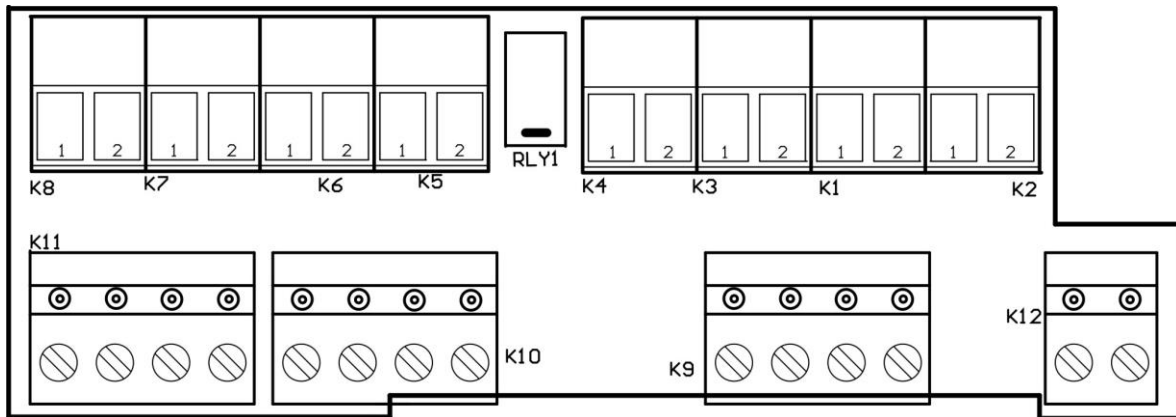
PCB Overlay
