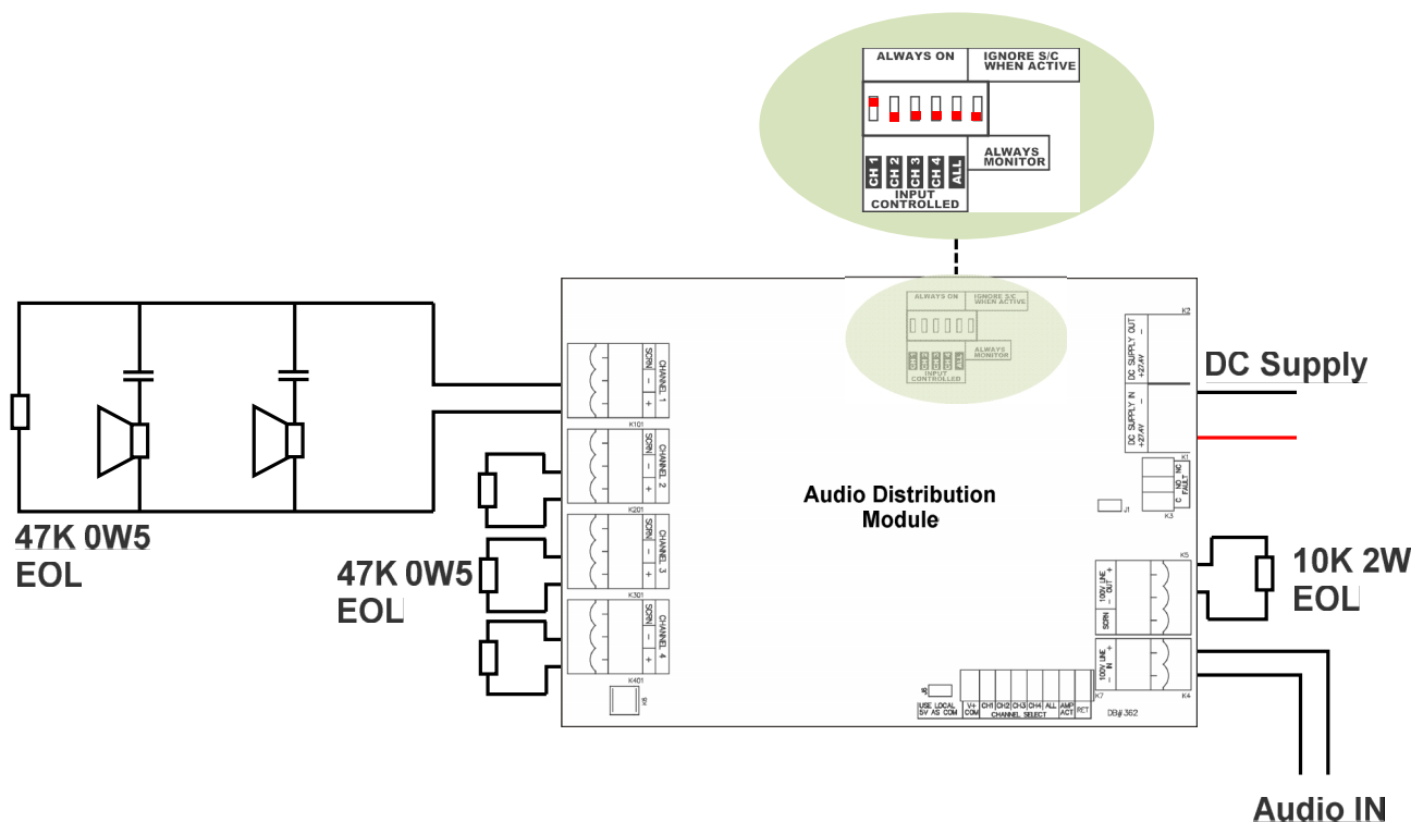
Figure 4: Basic Connection 4 Monitored Channels
