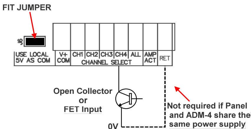
Figure 2: Open Collector or Open Drain Using Local 5V Supply (Common 0V required)
