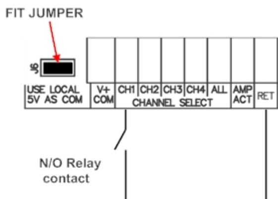
Figure 1: Relay Contact
