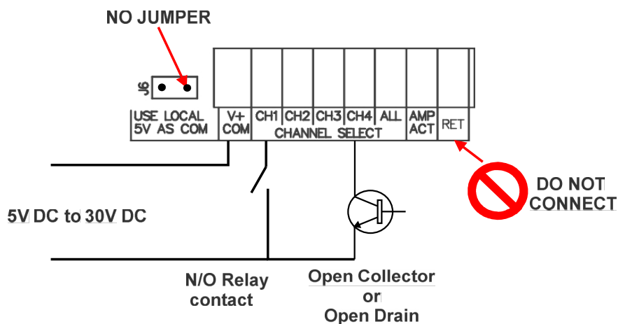
Figure 3: Using Isolated Supply
