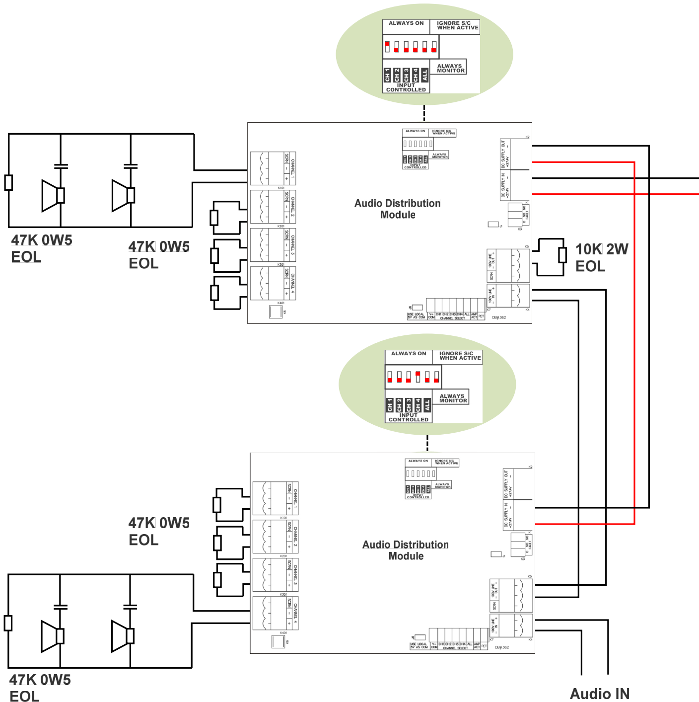
Figure 5: Multiple Audio Distribution Modules
