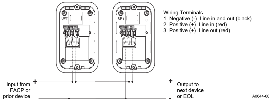
Figure 7 System Wiring
