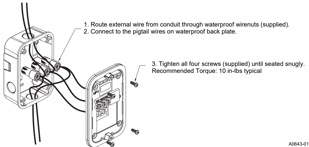
Figure 6 Wiring Terminals and Wire Leads
