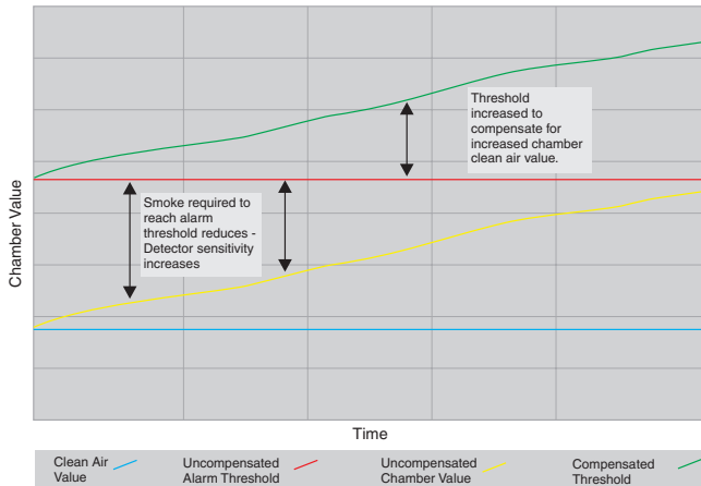
Figure 7: Dust Build up and Drift Compensation
