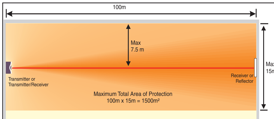
Figure 2c: Maximum Area Coverage for Beam Detectors
