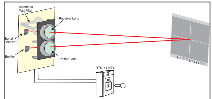
Figure 9: 6500 Beam Detector Asuretest Operation
