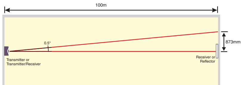
Figure 6: Effect of Detector Movement
