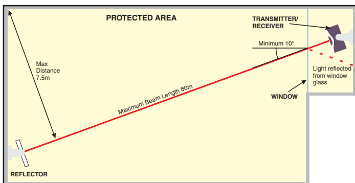
Figure 4: Reflective Beam Detector Operating through a Window.
