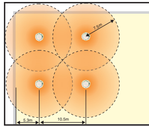
Figure 2a: Maximum Area Coverage for Point Detectors
