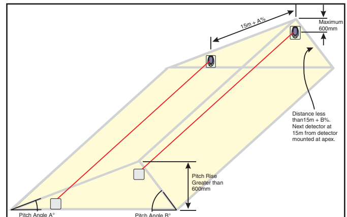
Figure 5: Beam Detector Mounting in Pitched Roofs.
